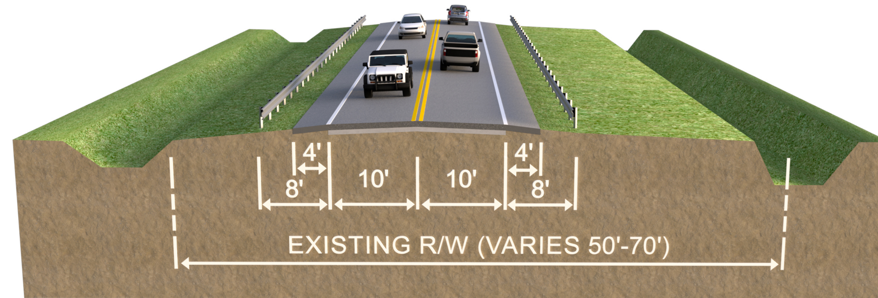
From Lonesome Island Road to west of Harney Pond Canal and east of the Indian Prairie Canal to CR 721 (Facing East)
