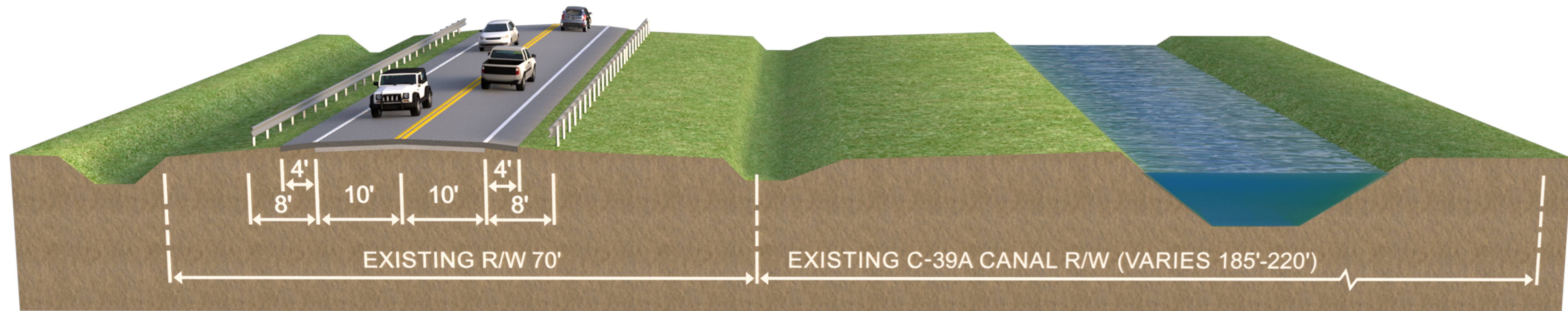
From west of Harney Pond Canal to east of the Indian Prairie Canal (Facing East)
