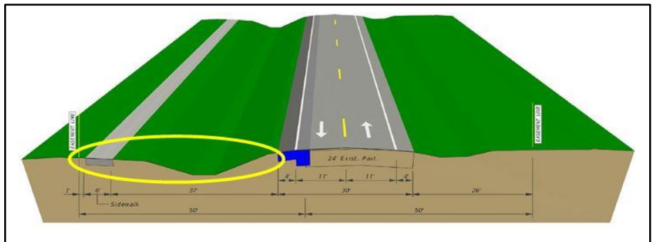
Typical section showing a new drainage ditch and 6' concrete along the western right-of-way line.
