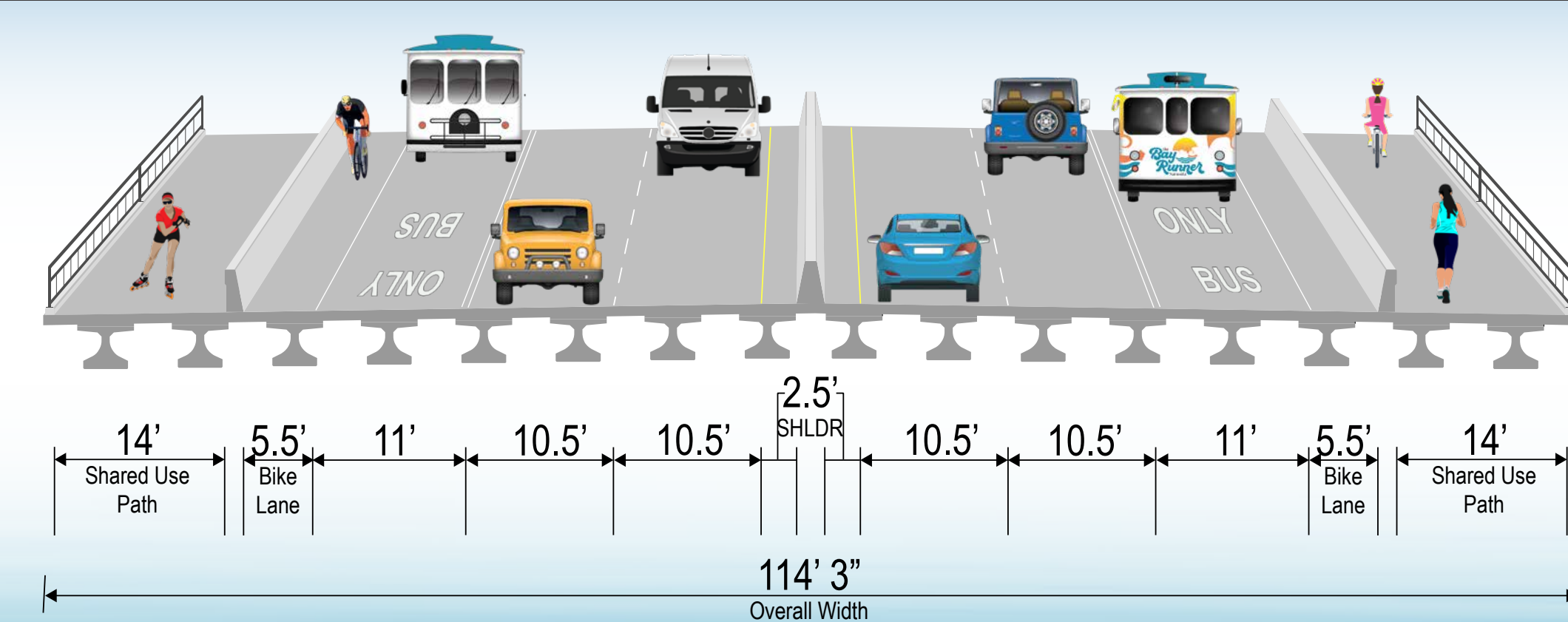
PROPOSED SINGLE BRIDGE TYPICAL SECTION
